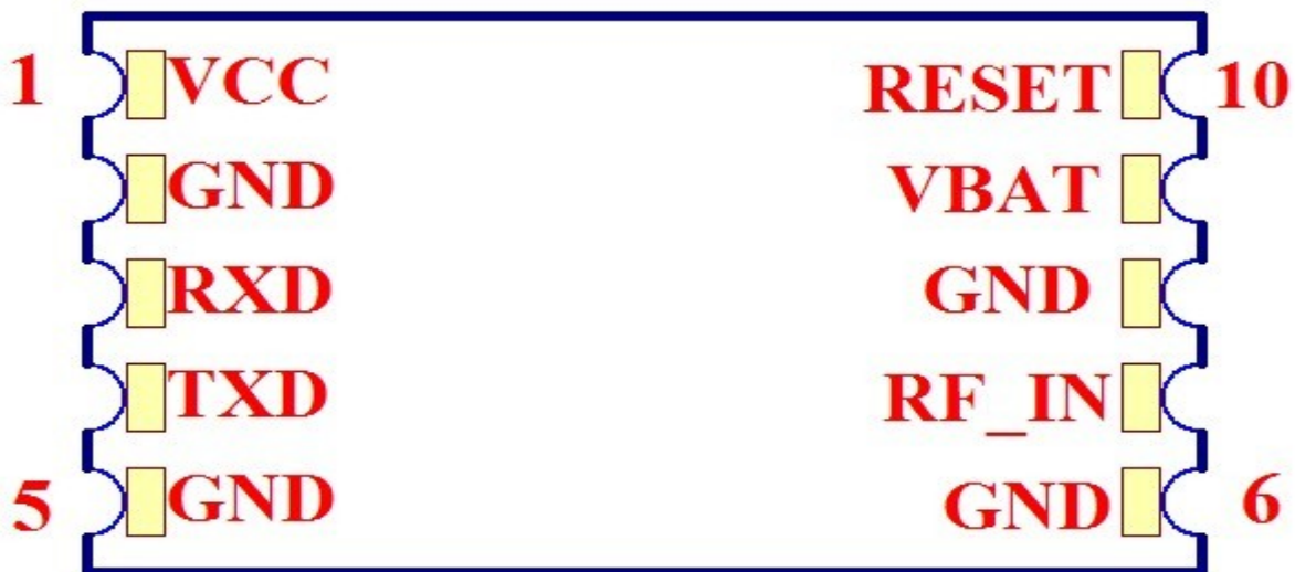
Figure 2: SM1108-MTBD Pin Package
