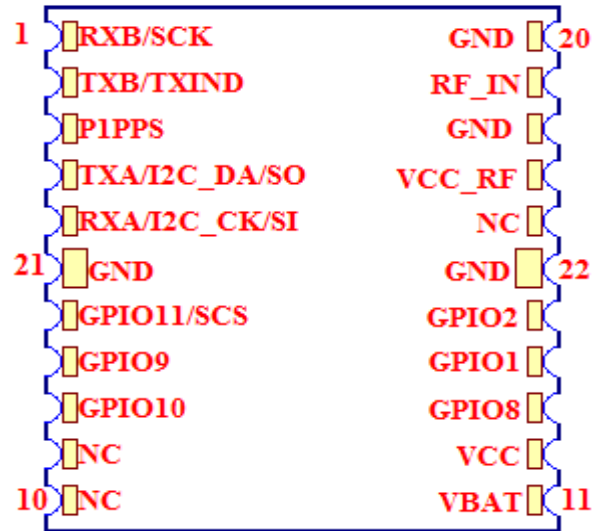
Figure 2: SM1513-MTBD Pin Package
