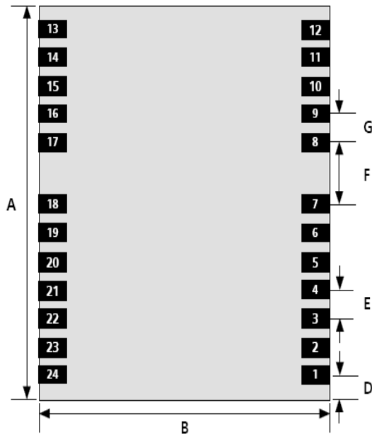
Figure 3: SM1612-MTBD Dimensions
