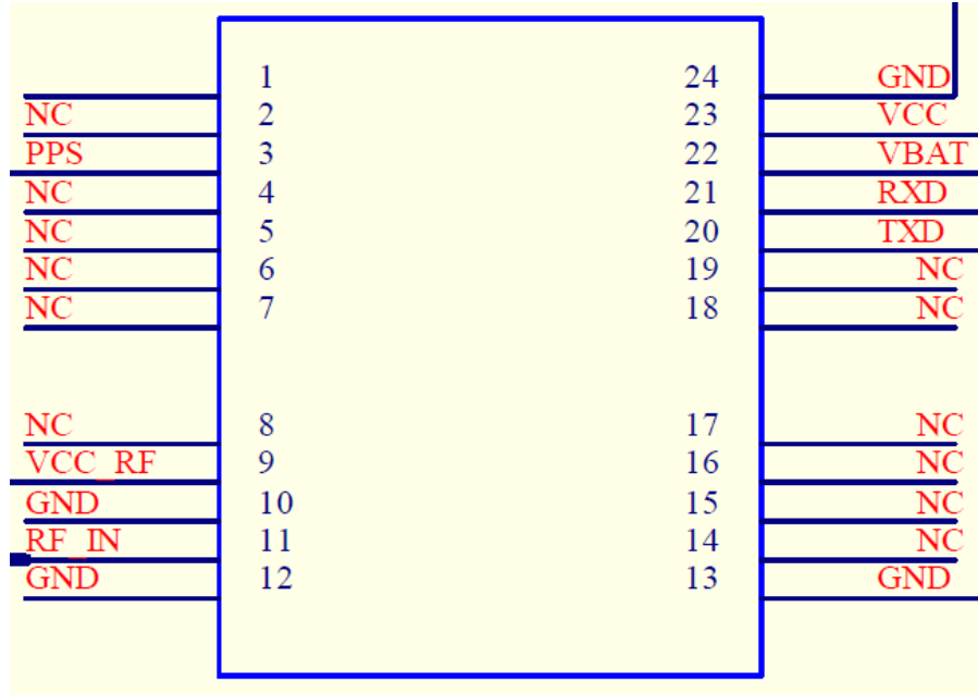
Figure 2: SM1612-MTBD Pin Package
