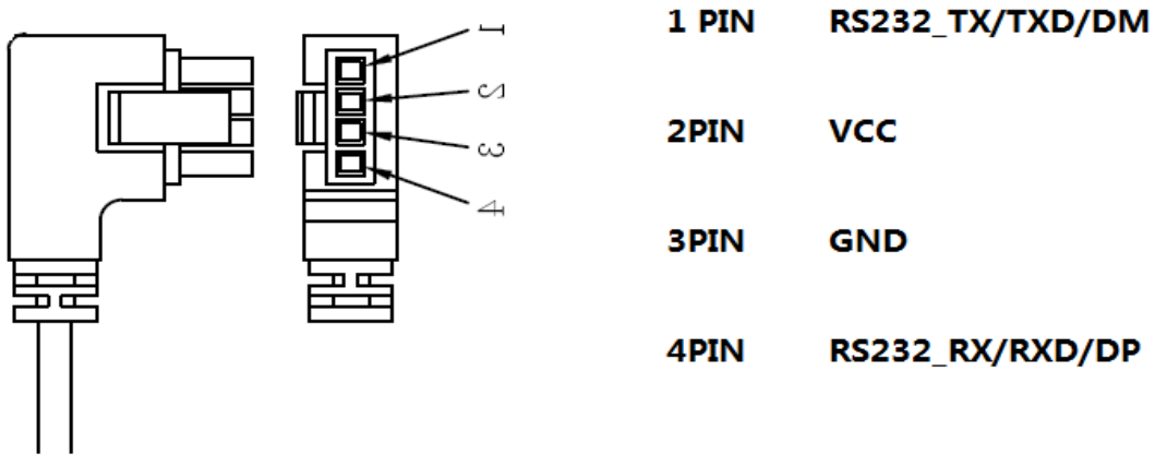
Figure 2: Molex 4pin Connector View
